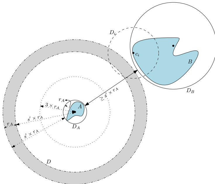
Figure 1: Illustration of Lemma 3.
