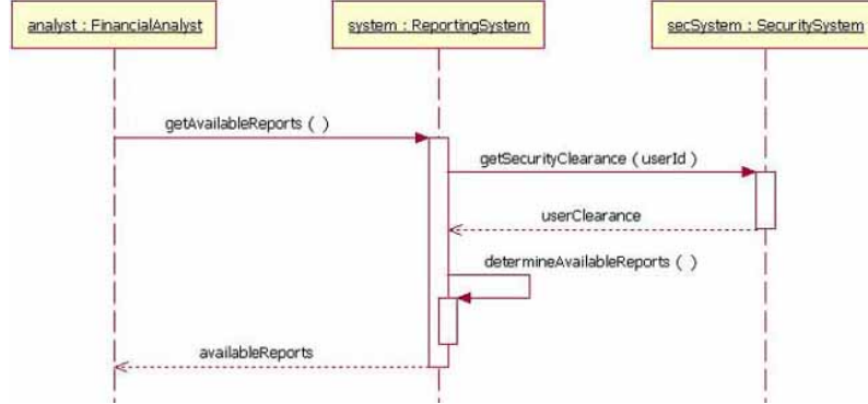
Figure 5: The system object calling its determineAvailableReports method
