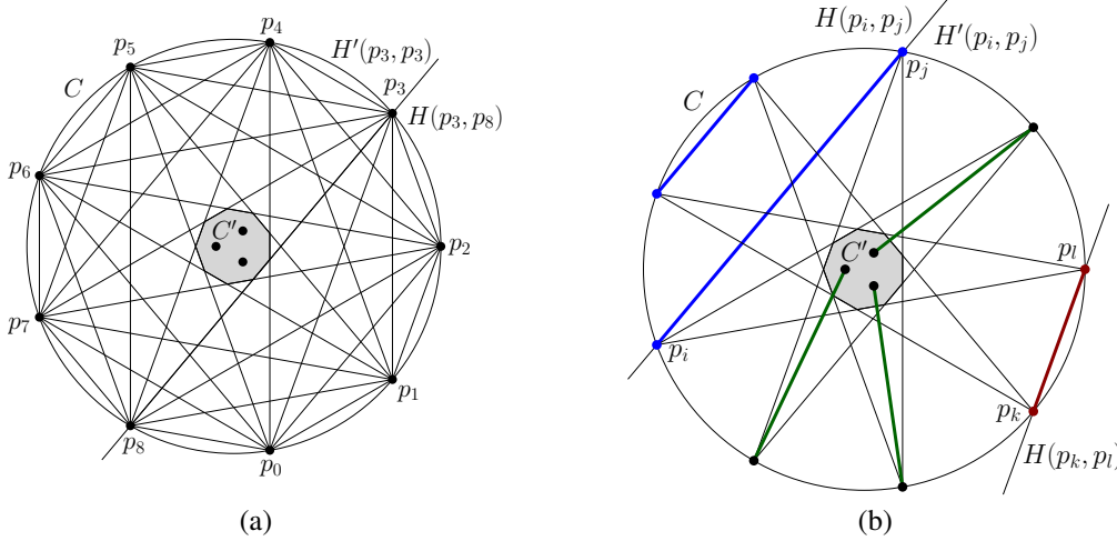
Fig. 3: (a) A variation of the regular wheel configuration. (b) Illustration of Lemma 2. The points of A and the edges of M(A) are in blue, and the points of B and the edges of M(B) are in red.
