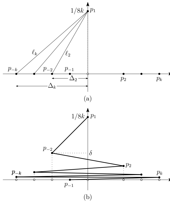
■ Figure 2 Illustration of the construction of a longest path for 2k points. The figure is not to scale as the real y -coordinates are very small so that the points lie almost on the x -axis. (a) Lifting p_1 to the y -coordinate 1/8k . (b) The final longest path.
