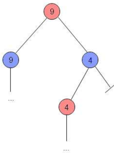
Figure 2: Alpha-Beta Pruning Example
