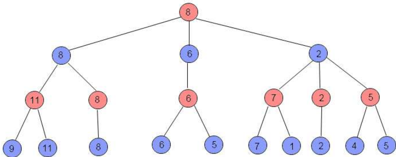
Figure 1: Sample Mini-Max Tree
