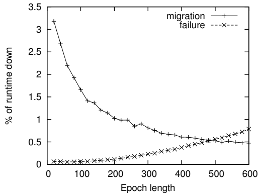
Figure 7.9: Downtime due to failure and preemptive migration at different lengths of scheduling epoch
