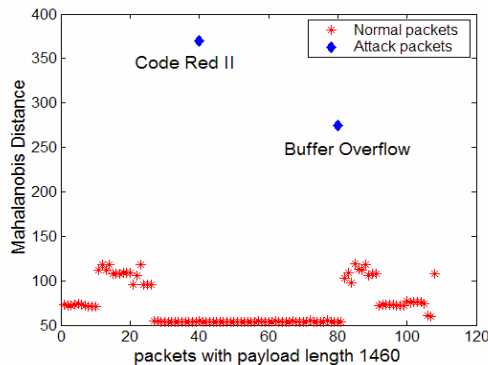
Figure 7. The computed Mahalanobis distance of the normal packets and the attacks, at length 1460.
