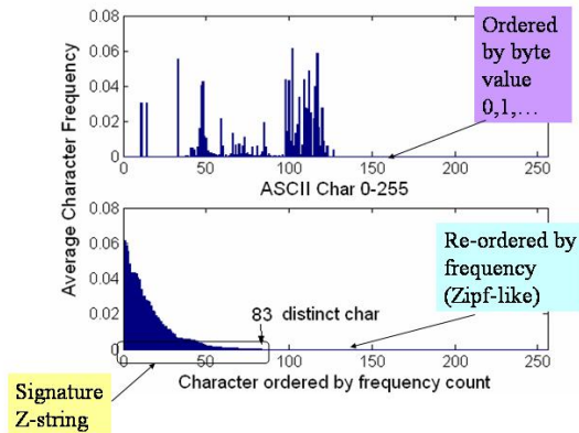
Figure 4. Payload distribution appears in the top plot, re-ordered to the rank-ordered count frequency distribution in the bottom plot. Notice there are only 83 distinct characters used in the average payload for this service (port 80, http) for this length distribution of payloads (all payloads with length 185 bytes).
