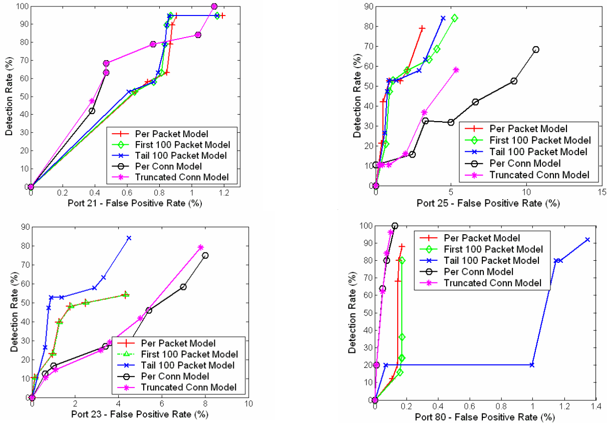
Figure 6. ROC curves for ports 21, 23, 25, 80 for the five different models. Notice the x-axis does not span to 100%, but limited to the worst false positive rate for each plot.
