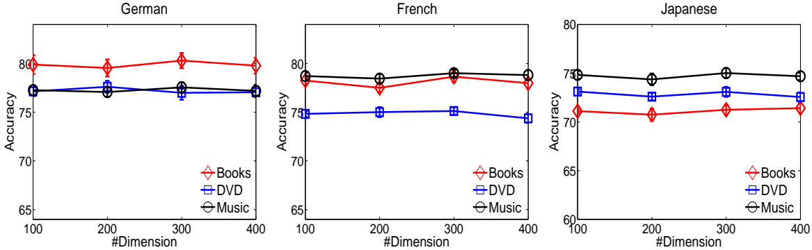
Figure 2: Average classification accuracy and standard deviation results for the proposed approach over 10 runs with respect to different dimensionality for the induced cross-lingual representations.
