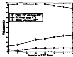
Fig. 13. Bottleneck utilization
