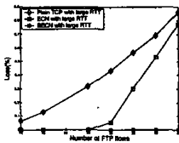
Fig. 12. Loss - Homogeneous flows
