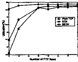
Fig. 6. Bottleneck utilization
