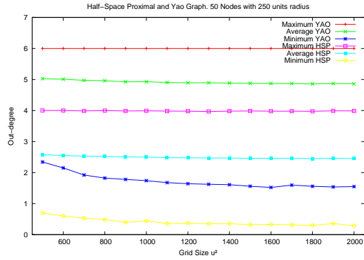
(b) Out-degree
