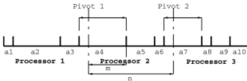
Figure 4: Data partitioning and pivots .
