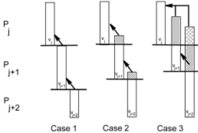
Figure 3: Illustration of cases for Merge\text{-}Subcube(DC_j) .
