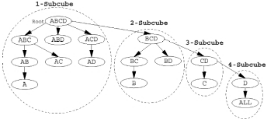
Figure 2: Subcubes of a data cube for d=4 .
