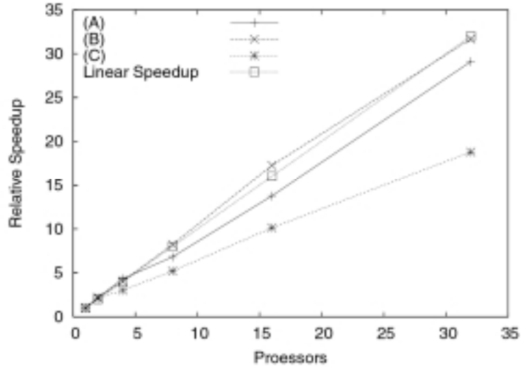
Figure 19: Relative speedup corresponding to Figure 18.
