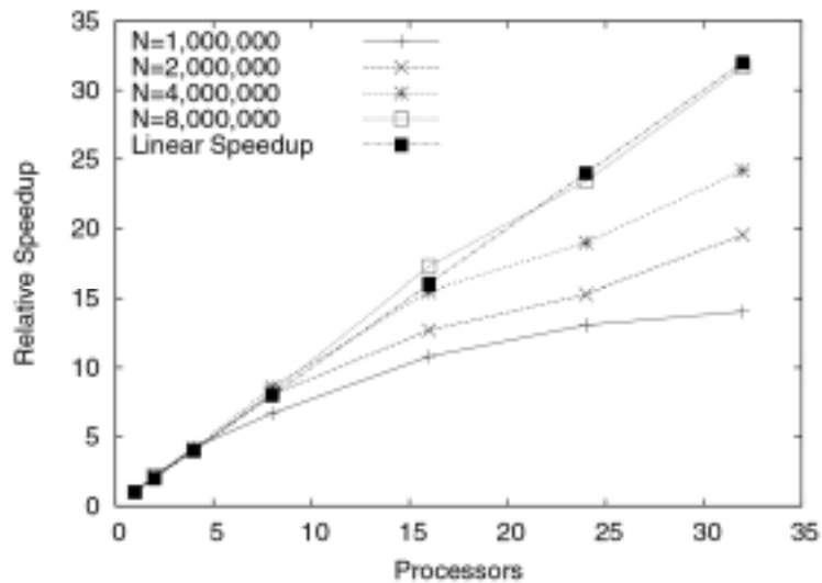
Figure 9: Relative speedup corresponding to Figure 8.
