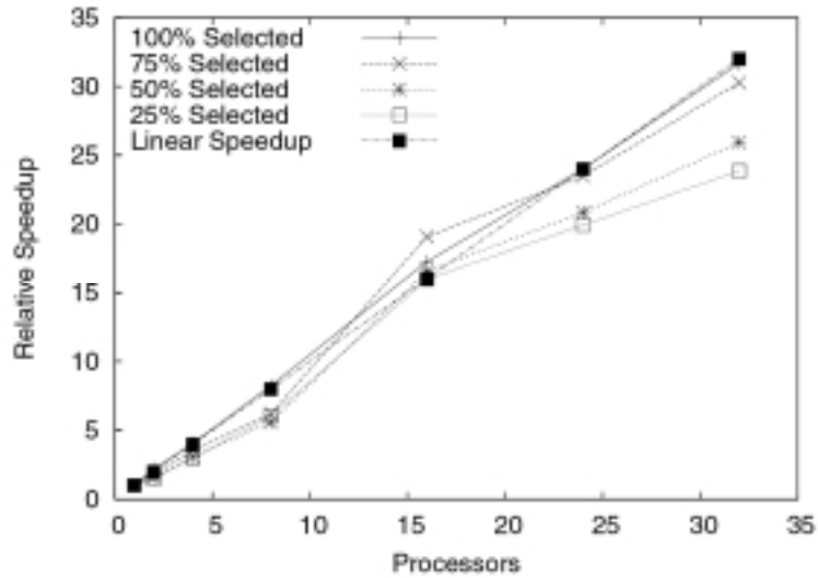
Figure 11: Relative speedup corresponding to Figure 10.
