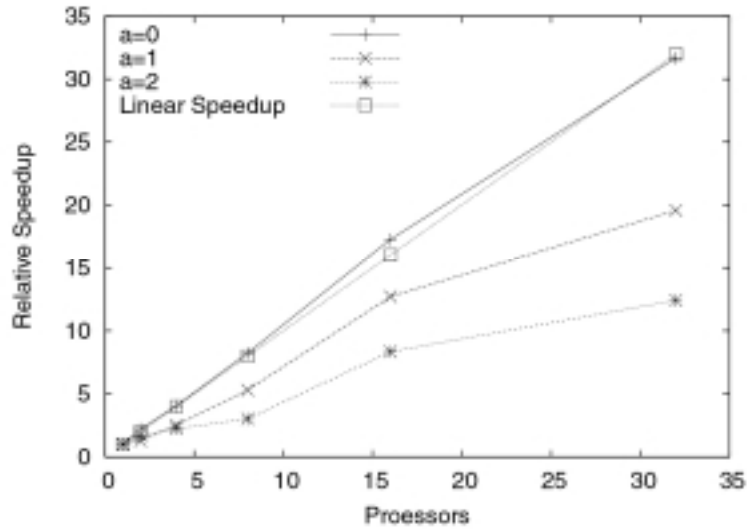
Figure 17: Relative speedup corresponding to Figure 16.
