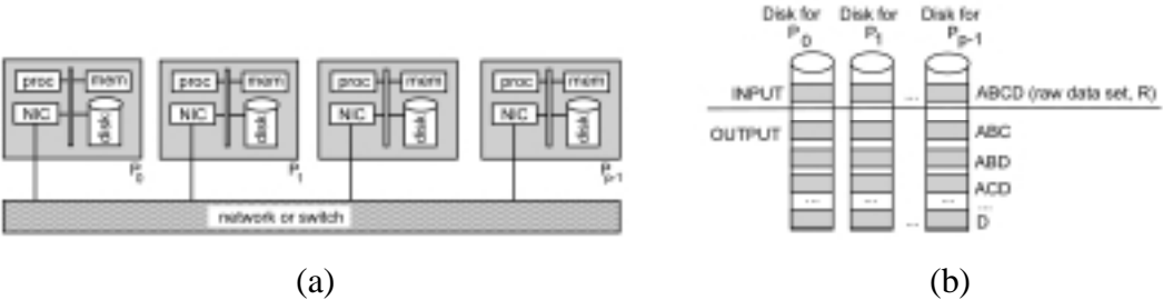
Figure 1: (a) Shared-Nothing Multiprocessor. (b) Data Partitioning.
