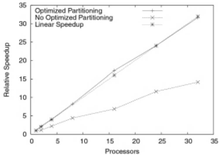
Figure 6: Relative speedup corresponding to Figure 5.
