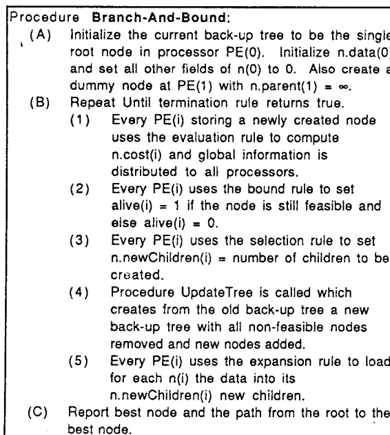
Figure 4. The Global Structure of the Branch-And-Bound Algorithm
