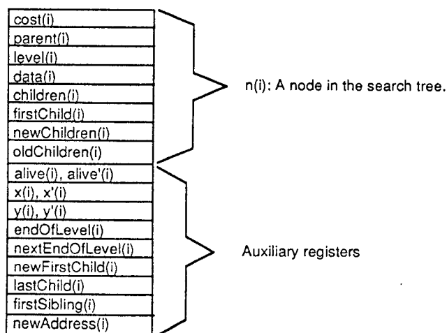
Figure 2. The Registers Required at Each Processor PE(i) .
