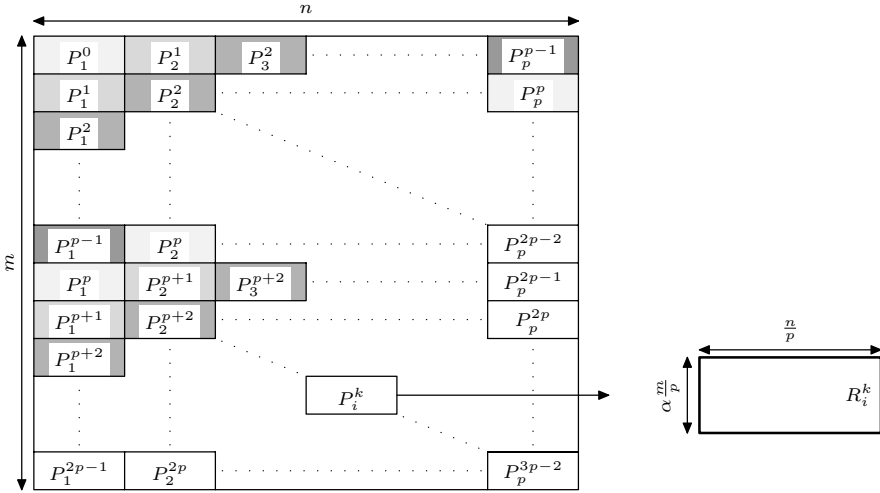
Fig. 4. An O(p) rounds scheduling with \alpha = 1/2
