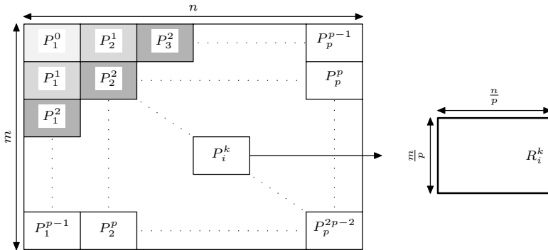
Fig. 3. An O(p) communication rounds scheduling with \alpha = 1
