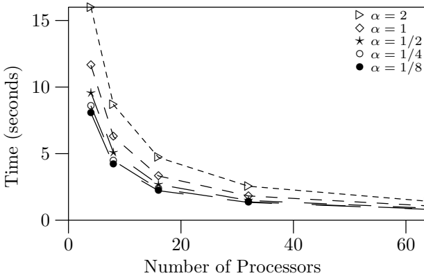
Fig. 5. Curves of the observed times for m = 8196 and n = 16384
