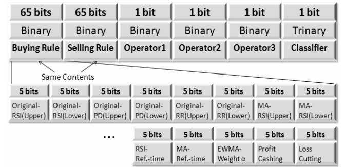
Fig. 2 A Chromosome Design
