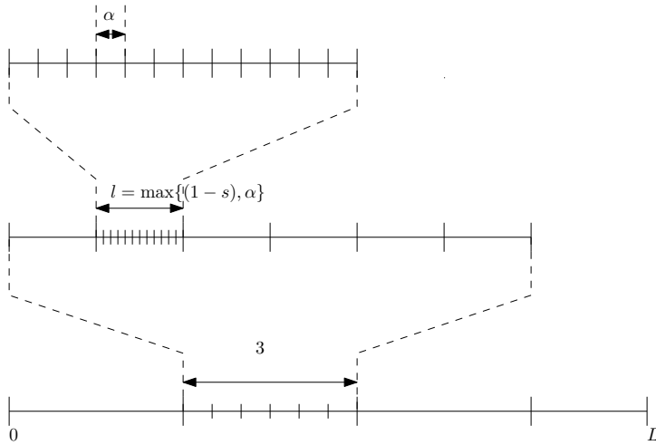
Figure 1: Partition \mathcal{P}
