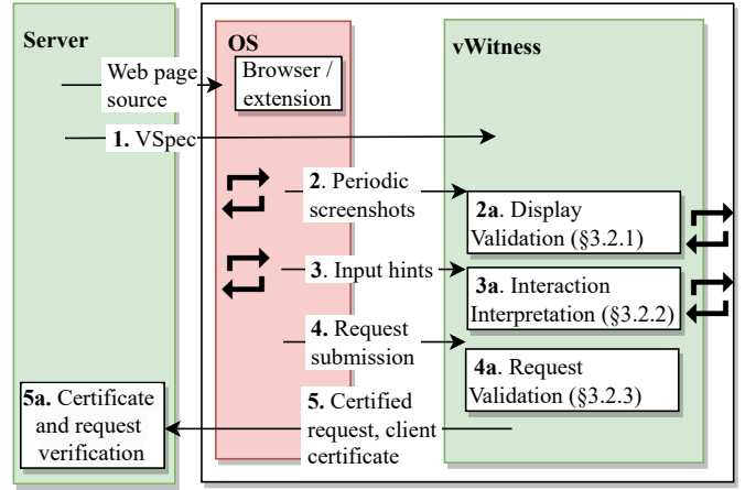
Figure 4: vWitness overview (§III). Green/red indicates trusted/untrusted entities.
