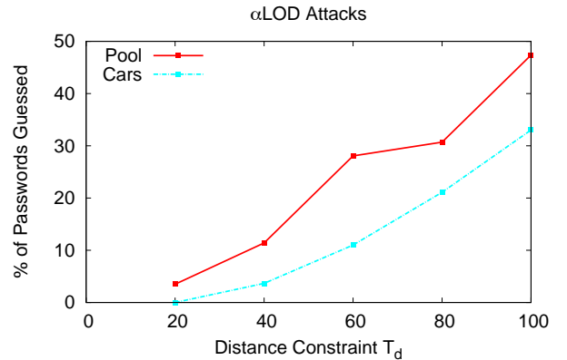
Fig. 10. \alpha LOD attacks: passwords guessed as a function of distance constraint T_d .
